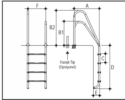
AS-METREK
