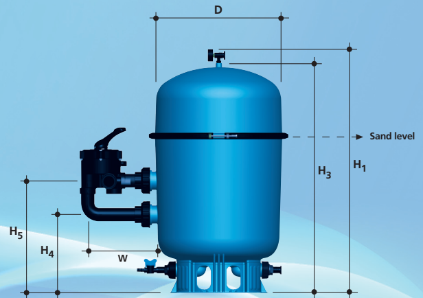
Sand water discharge openings are available at both front and rear, installed with discharge valve.
