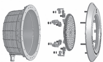
SlimLED Light Installation in the niche
